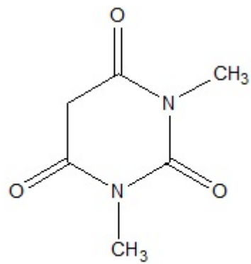
1,3-Dimethylbarbituric acid
